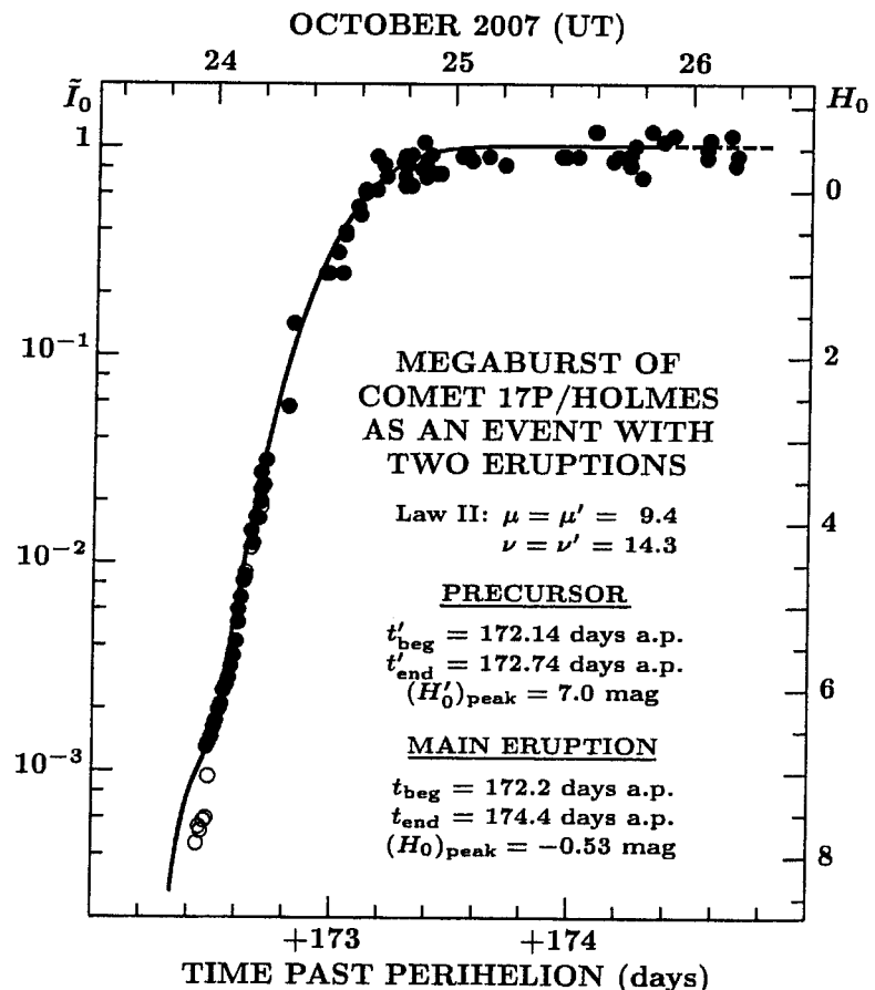
Figure 6. Curve of intrinsic brightness of comet 17P/Holmes during the megaburst, fitted as a double-eruption event. The precursor, a relatively minor outburst, is followed and overlapped by the main eruption. The precursor is responsible for a wiggle in the slope of the curve near the faintest magnitude data based mostly on Henriquez Santana's (2008) frames with unsaturated images. The primary parameters of the two eruptions are listed; for more information, see Table 5 and the caption to Figure 4.
