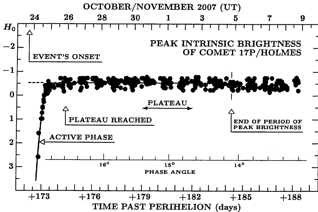
Figure 3. Close-up view of the temporal variations in the intrinsic magnitude H_0 following the active phase of the 2007 megaburst of comet 17P/Holmes. The peak intrinsic magnitude (H_0)_{\text{peak}} = -0.53 \pm 0.12 has been calculated from 291 magnitude estimates that make up the flat portion of the plateau, between 174.4 and 184.3 days after perihelion, or between October 25.9 and November 4.8 UT. These boundaries have been determined in part from the sets of averaged values of H_0 in Table 2. The beginning of the plateau with the peak intrinsic brightness coincides with the termination time of the active phase of the megaburst. Variations in the phase angle are also shown.
